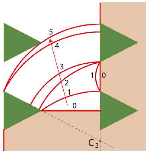
Figure 9: (color online) Upward motion of a kink in an elastic wall (red online).
