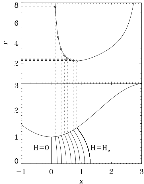
Figure 3: Construction of the metastable elastic lines bounded between 0 and f(x) = 2 - \cos(x) , as a function of the external field or arc radius. We depict the boundaries and the metastable walls for different fields H in the lower plot. In the upper plot we represent the function [f(x)/f'(x)]\sqrt{1 + f'(x)^2} . The intersection of the arc radii r = \sigma/(2H) with this function gives the upper contact point (x_1, f(x_1)) of the metastable wall with the top border f(x) . The depinning field is H_c , above which there are no metastable states.
