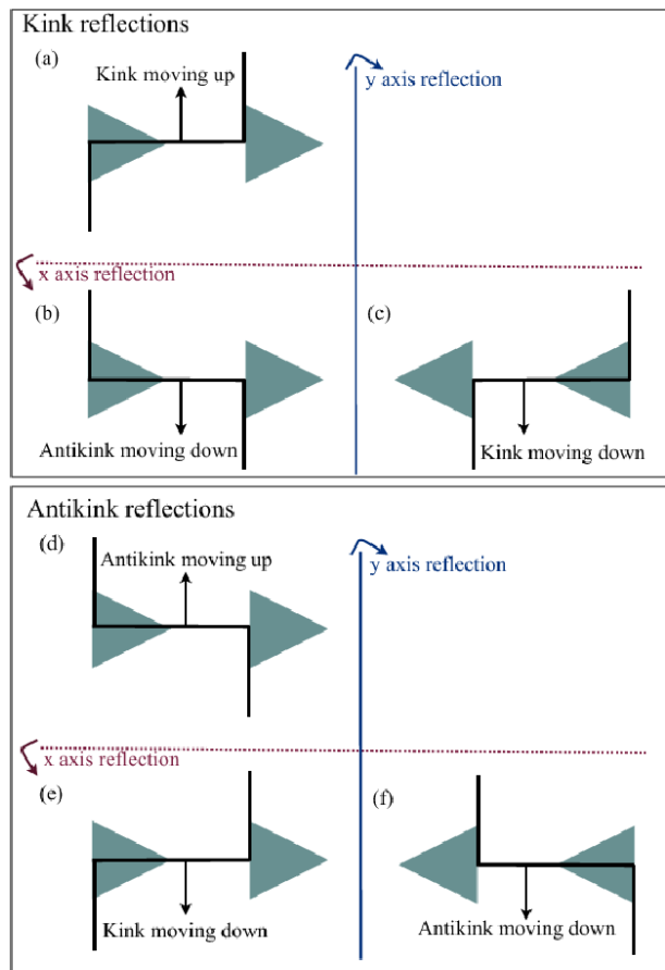
Figure 6: (color online) Broken symmetry in a 2D kinked wall. (a) Kink moving up. (b) After an x-axis reflection, an antikink moving down is obtained. (c) After a second y-axis reflection, a kink moving down on a different array (inverted triangle array) is obtained. From (d) to (f) same reflections are shown for an antikink.
