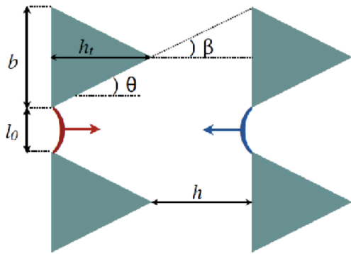
Figure 5: (color online) A two dimensional ratchet geometry made by triangles.
