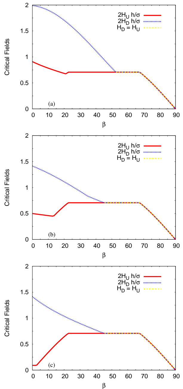
Figure 10: Critical fields, H_D and H_U normalized by \sigma/2h vs. \beta calculated for \theta = 45^\circ for (a) h/l_0 = 10 (b) h/l_0 = 1 and (c) h/l_0 = 0.1 . Note that for large \beta , H_D becomes equal to H_U and, therefore, a single line appears in the figures.
