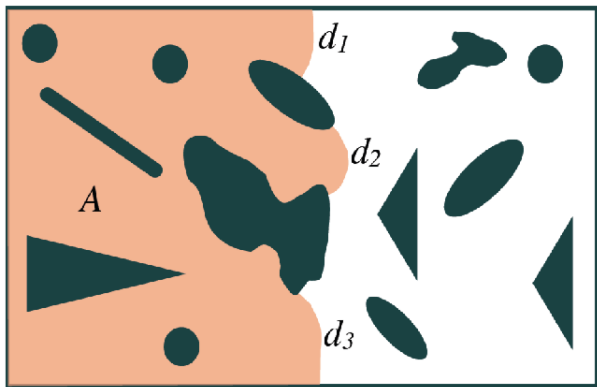
Figure 1: (color online) Interface in a two dimensional medium with free holes and sample boundaries. The gain of interface energy by optimally intersecting the holes and sample boundaries produces domain wall pinning.
