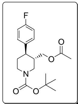
(3 S ,4 R )- 2d
