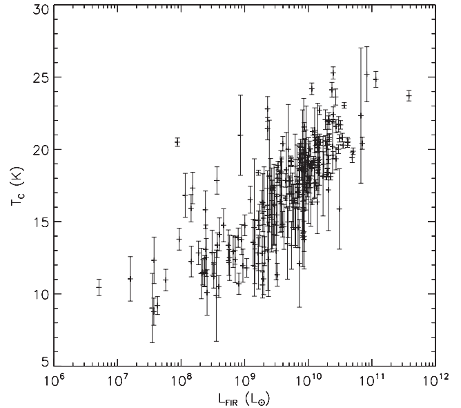
Figure 20. Temperature of the cold dust component versus the IR luminosity (40–1000 \mu\text{m} ) in the two-component grey body fits.
