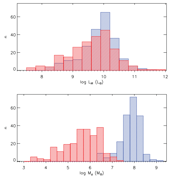
Figure 3. Distributions of the total IR luminosity (3–1000 \mu\text{m} ) and dust mass for the warm (red) and cold (blue) dust components of the MAGPHYS fits.
