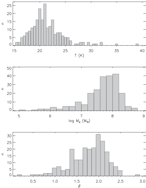
Figure 14. Distributions of temperature, mass and \beta for single-temperature grey body fits to our sample galaxies. The values are the results of fits to data at wavelengths between 100 and 850 \mu\text{m} (353 GHz) inclusive.
