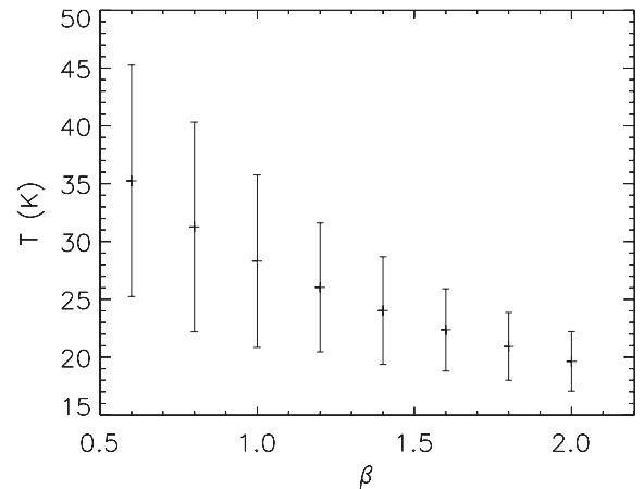
Figure 15. Median and standard deviation of the temperature distributions for single-component-modified blackbody fits in which \beta is fixed at various values.
