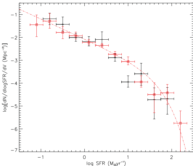
Figure 12. SFR function. The black symbols show the function obtained from the MAGPHYS-derived SFRs, while the red symbols relate to SFRs derived by scaling the total IR luminosities by a constant ( 1.5 \times 10^{-10} ; Kennicutt & Evans 2012), see also equation 4.
