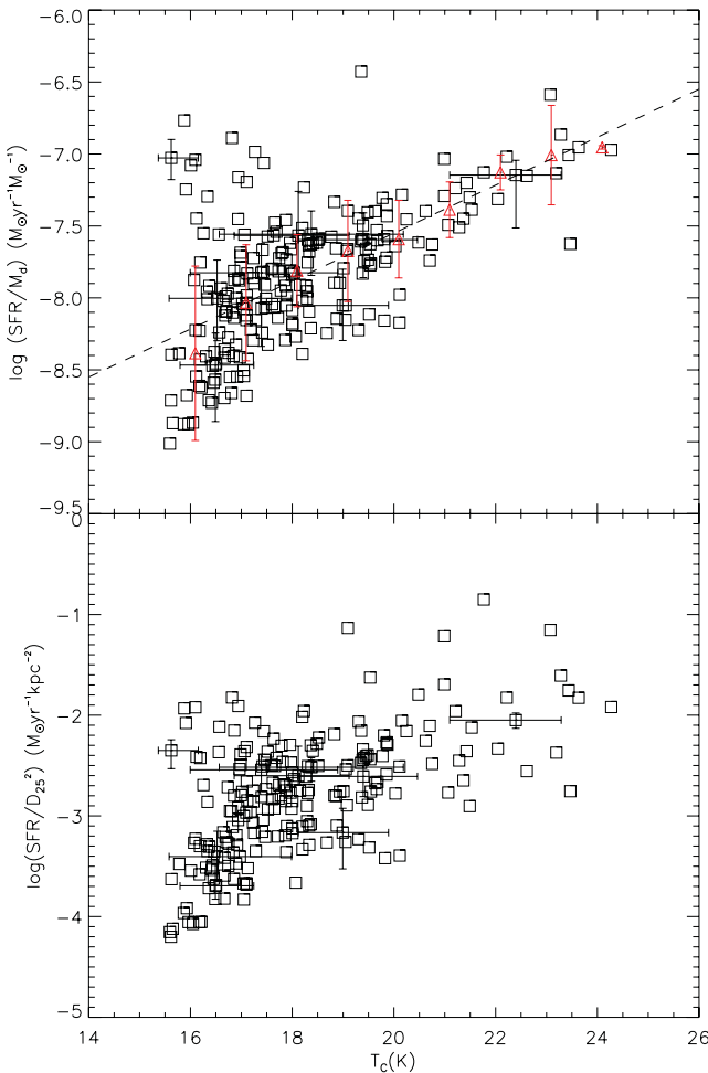
Figure 8. Top: SFR per unit dust mass as a function of the cold dust temperature. The dashed line is the least-squares linear relation. The red symbols indicate the median and the standard deviation in bins of temperature. Bottom: SFR surface density, estimated as the \text{SFR}/D_{25}^2 , as a function of the cold dust temperature. Only a few representative error bars are shown for each plot.
