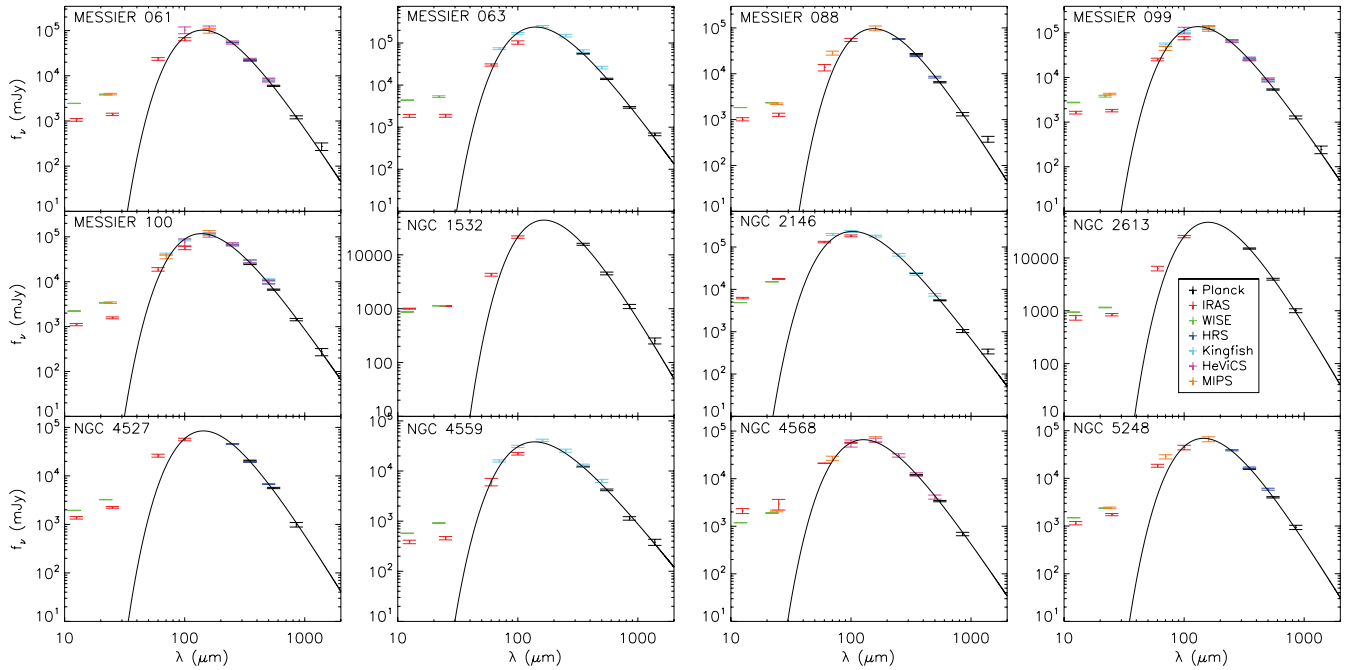
Figure 13. Some example single-temperature grey body fits. Only points at \lambda \geq 100 \mu\text{m} are taken into account in the fitting procedure (see the text).
