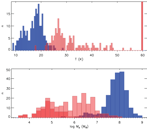
Figure 18. Distributions of temperature and mass for two-component grey body models with \beta fixed at 2. Values for the cold dust component are shown in blue, and those for the warm component in red. For 73 galaxies the temperature of the hot component was 60 K, the maximum allowed value. These objects are highlighted by darker red shading.
