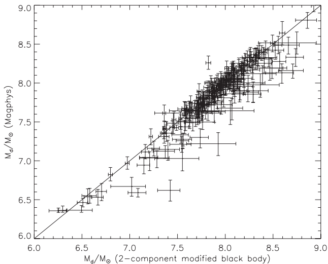
Figure 19. Comparison of dust masses derived from simple two-component grey body fits and those derived by MAGPHYS. The values from the latter have been multiplied by a factor of 2 to allow for the different values of the dust mass opacity coefficient, \kappa_d , used (see the text).
