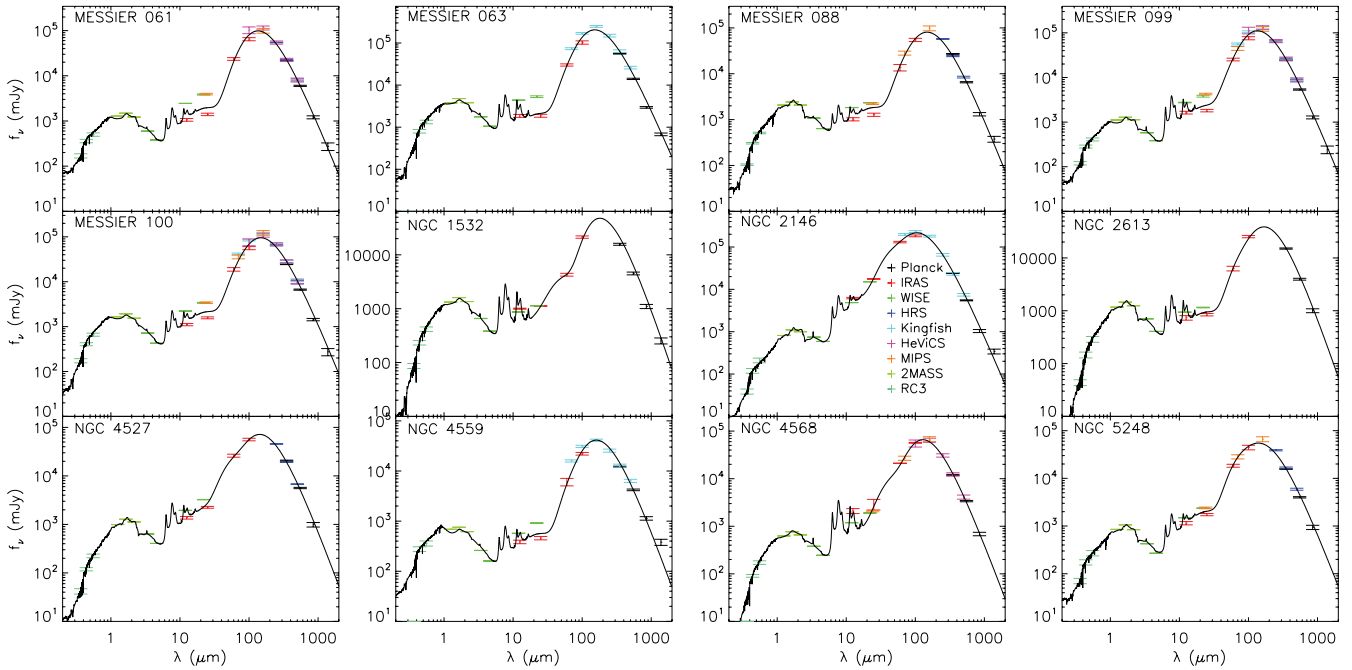
Figure 1. Some example best-fitting SED models produced by MAGPHYS.
