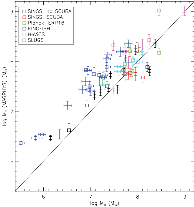
Figure 4. Comparison of our dust masses with those of other authors. Black: Draine et al. (2007), galaxies with no 850 \mu\text{m} SCUBA flux densities; red: Draine et al. (2007), galaxies with 850 \mu\text{m} flux densities; green: Planck Collaboration XVI (2011); blue: Skibba et al. (2011); cyan: Auld et al. (2013); magenta: Dunne et al. (2000) from two-component fits. Masses have been scaled to a common value of \kappa_{850\mu\text{m}} = 0.0383\text{ m}^2\text{ kg}^{-1} [necessary for Dunne et al. (2000) and Planck Collaboration XVI (2011)].
