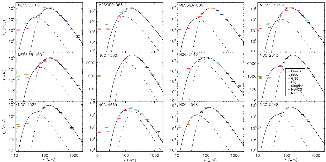
Figure 17. Some example two-component grey-body fits. Only points at \lambda \geq 60 \mu\text{m} are taken into account in the fitting procedure (see the text).
