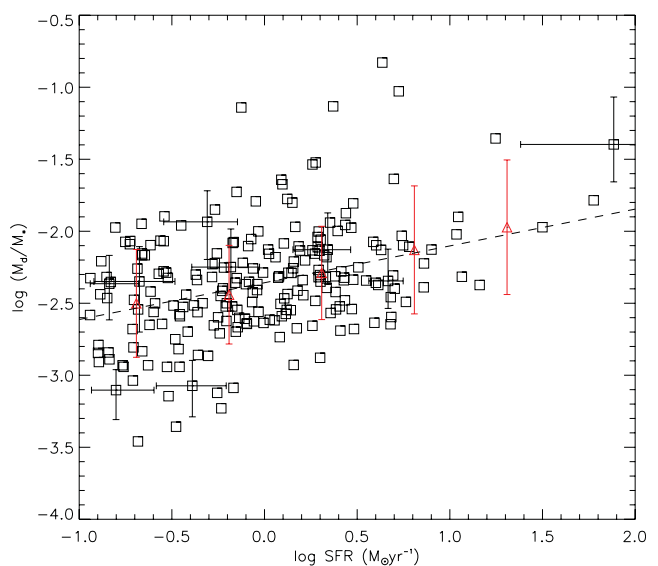
Figure 7. Dust mass per unit stellar mass as a function of the SFR. The dashed line is the least-square fit. The error bars are shown on only a small number of points for clarity. The red symbols indicate the median and standard deviation in bins of SFR.
