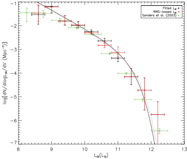
Figure 11. Total far-IR (3–1000 \mu\text{m} ) luminosity function calculated from the luminosity function at 545 GHz as presented in Negrello et al. (2013) and the MAGPHYS-derived far-IR luminosities. The black line shows the best-fitting Schechter function with parameters, \alpha = -1.78 \pm 0.18 , L_{\text{IR}}^* = 1.71 \times 10^{11} L_{\odot} and \phi^* = 3.60 \pm 1.72 \times 10^{-4} \text{ Mpc}^{-3} \text{ dex}^{-1} . The red symbols show the same luminosity function calculated using just the IRAS 60 and 100 \mu\text{m} flux densities and the green symbols show the luminosity function as derived by Sanders et al. (2003).
