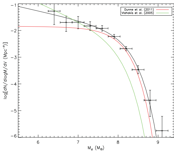
Figure 10. Dust mass function calculated from the luminosity function at 545 GHz as presented in Negrello et al. (2013) and the MAGPHYS-derived dust masses. The black line shows the best-fitting Schechter function with parameters given in Table 2. The red and green lines show the dust mass functions of Dunne et al. (2011) and Vlahakis et al. (2005) after scaling them to approximately account for the different value of \kappa_d used by these authors.
