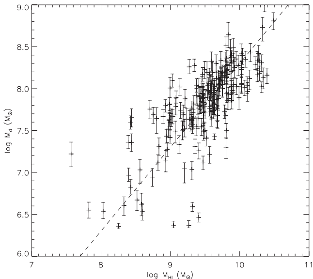
Figure 6. Correlation between total dust mass and atomic hydrogen mass. The straight line is for a ratio M_d/M_{H1} = 0.02 .
