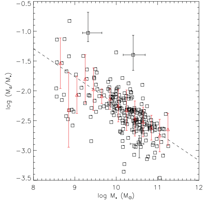
Figure 5. Ratio of dust mass to stellar mass as a function of stellar mass. The error bars are shown on only a small number of points for clarity. The median values in bins of stellar mass are shown in red, where the length of the error bars is the standard deviation within the bin. The dotted line is a least-squares fit to the binned points, excluding the bins with few points.
