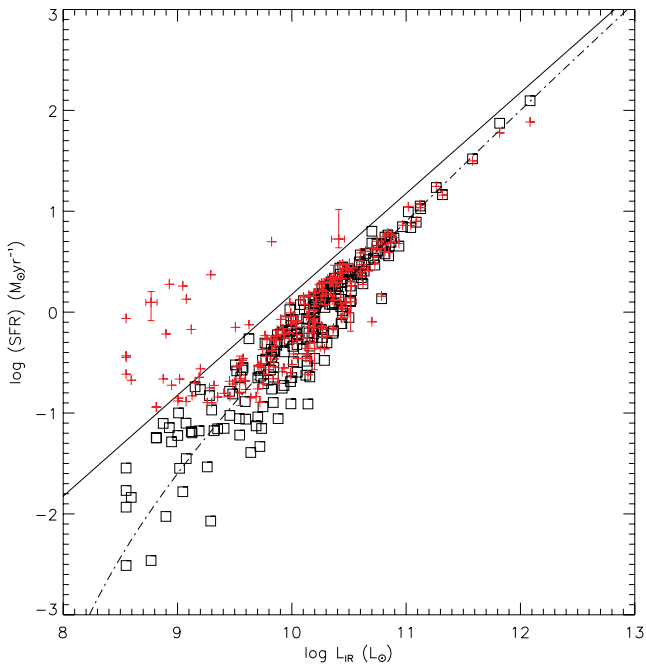
Figure 9. SFR as a function of the total IR luminosity, L_{\text{IR}} (3–1000 \mu\text{m} ). The black squares are the SFR that would be obtained by using the IR luminosity of the warm dust component in equation (4), whereas the solid black line shows the SFR that would be obtained by using the total IR luminosity in equation (4). The red symbols are the SFRs as derived by MAGPHYS.
