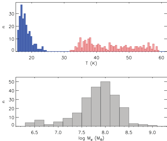
Figure 2. Distributions of temperature and dust mass for MAGPHYS fits.
