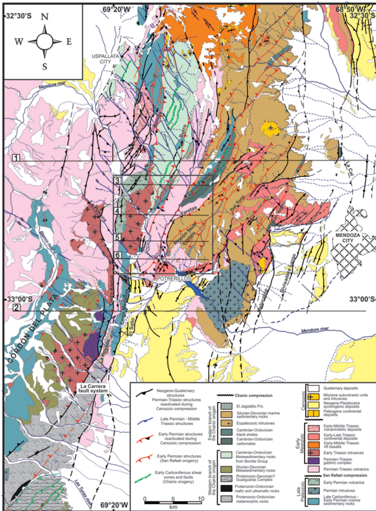
Fig. 2.- Geological-structural map of the Southern Precordillera and the Cordon del Plata range (modified from Giambiagi et al. , 2011 and Heredia et al. , 2012). The different colors in the structural traces represent different deformational phases. The box indicates the Quebrada de La Polcura and Quebrada del Medio area. Dotted lines with numbers are the traces of cross-sections (see Figs. 3 and 5B).
