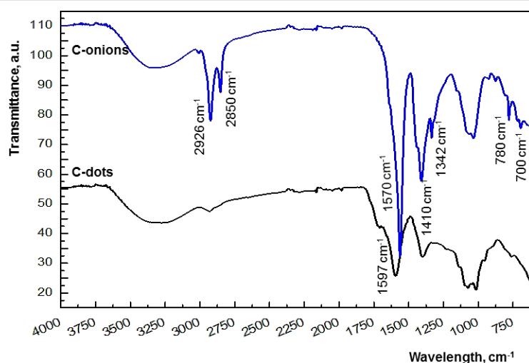
Figure 5: FTIR spectra of C-dots and C-onions obtained by carbonization of tomatoes in aqueous solution and NaOH 30% (w/v), respectively.
