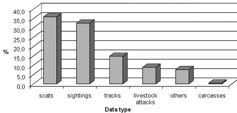
Figure 2. Frequencies of the different types of data (n = 237) recorded during the 2000–2014 period.
