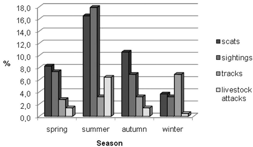
Figure 4. Seasonal distribution of the different types of data (n = 218).
