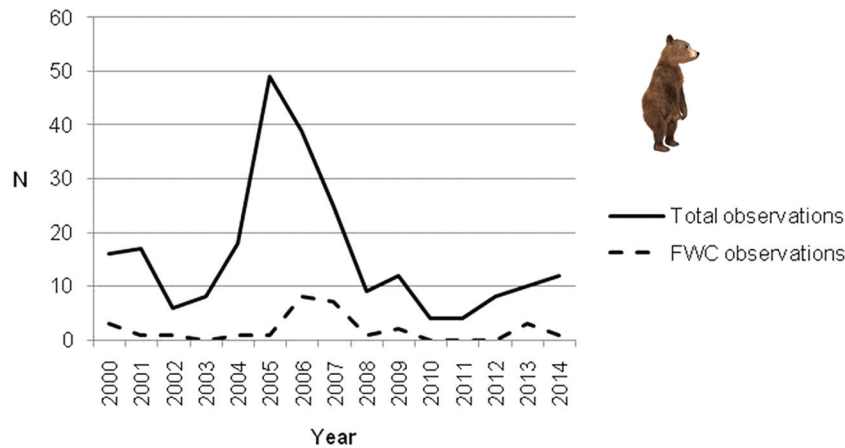
Figure 6. Number of total observations (n = 237) and observations of females with cubs (FWC, n = 29) per year. Picture copyright: Valentyna Chukhlybova, Image ID: 39802292, http://www.123rf.com .
