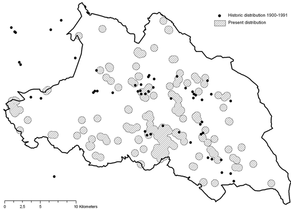
Figure 3. Comparison of the historic (1900–1991 period, n = 61; Boscagli et al. 1995) and current (n = 237) distribution of brown bear data the in study area and surroundings.
