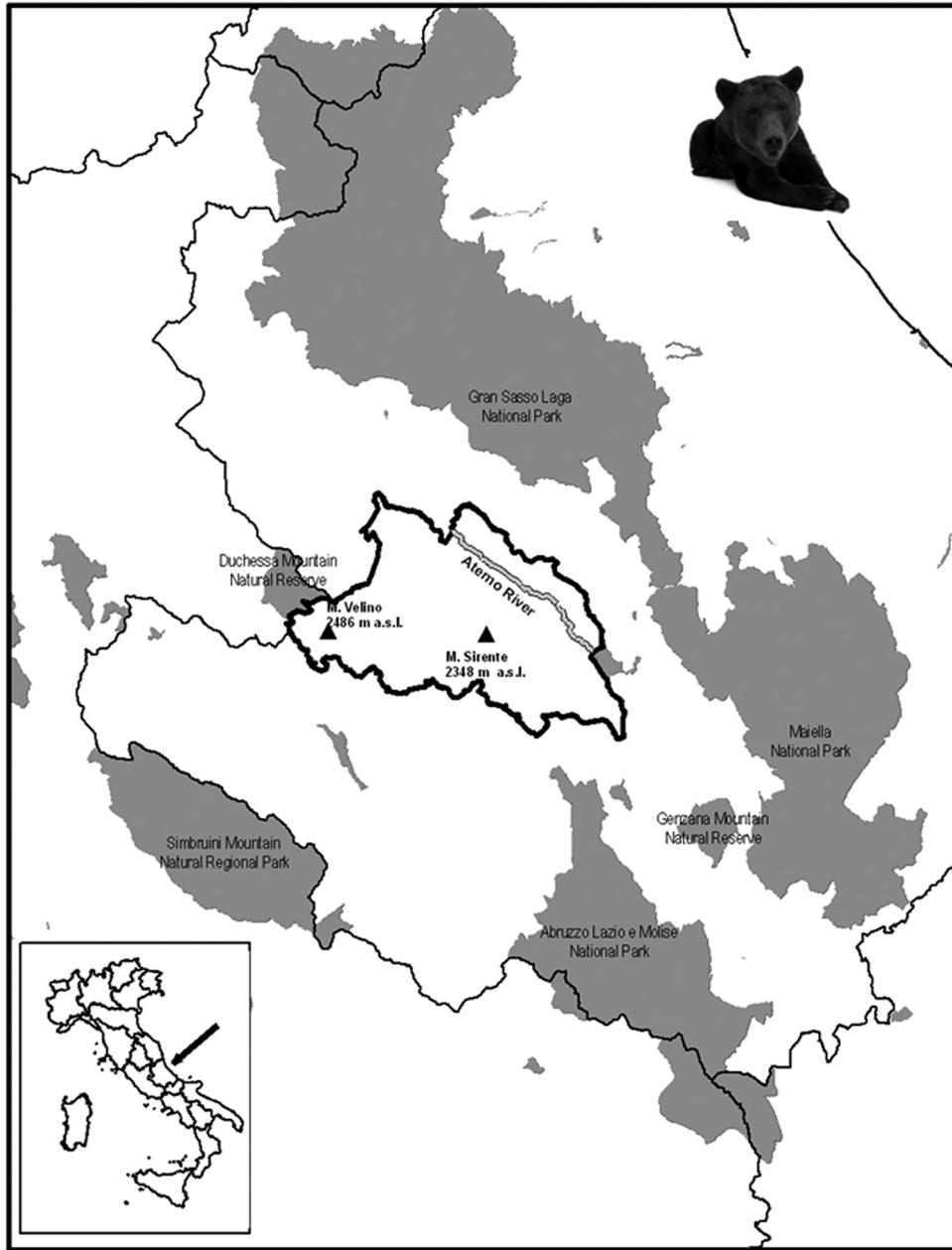
Figure 1. The study area (ZPS Sirente Velino-IT7110130) and neighboring protected areas. Picture copyright: Eric Isselee, Image ID: 7980363, http://www.123rf.com .
