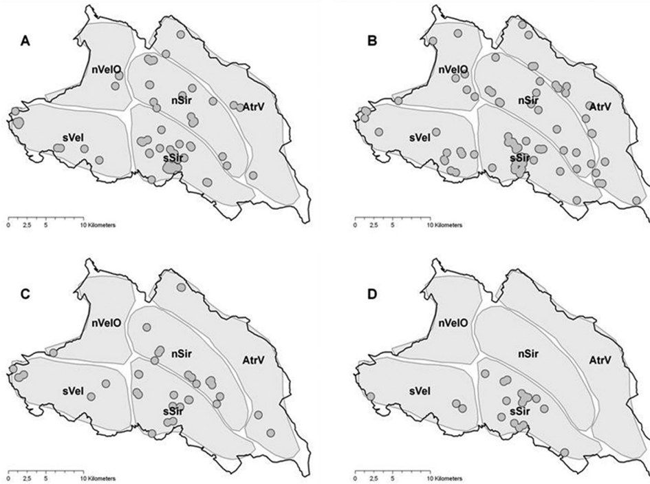
Figure 5. Distribution of data type collected (n = 218) in the study area blocks (see text for more details): (A) scats; (B) sightings; (C) tracks; and (D) livestock attacks. sSir: south Sirente; nSir: north Sirente; AtrV: Aterno River Valley; sVel: south Velino; nVel: north Velino.
