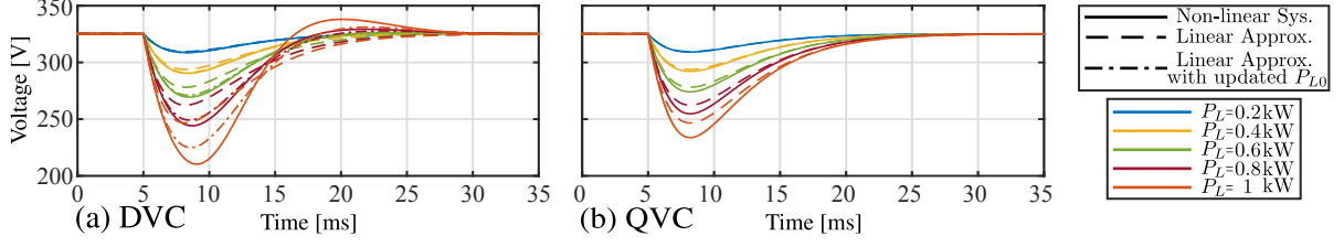
Fig. 3: Non-linear simulated response compared with the linear approximation of \frac{\Delta V(s)}{\Delta P_L(s)} under increasing active power steps. (a) DVC; (b) QVC. Results using the data in Table I.
