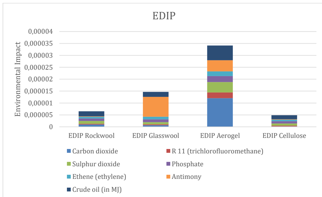
Figure 26 EDIP Results
