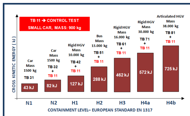
Figure 1. Containment levels for security barriers [EN 1317-2 (2011)].
