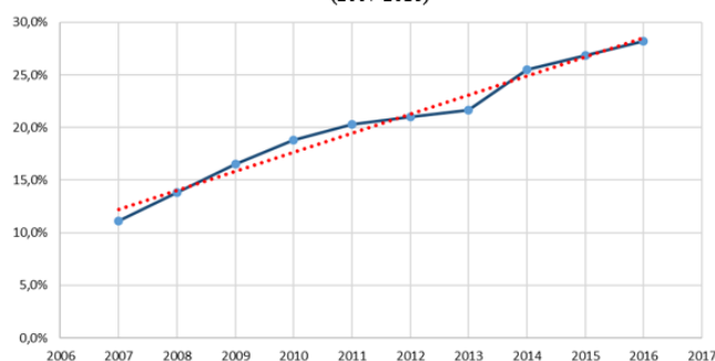
Figure 2. Evolution of light vehicles in the fleet in Spain (2007-2016)
