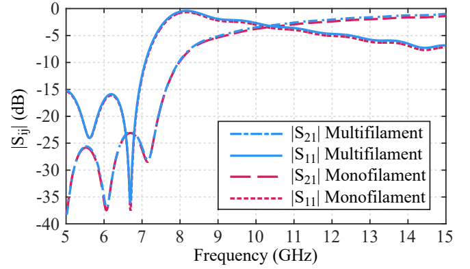
Figure 11: Comparison of the simulated scattering parameters of the equivalence between conductive multifilament and monofilament threads.
