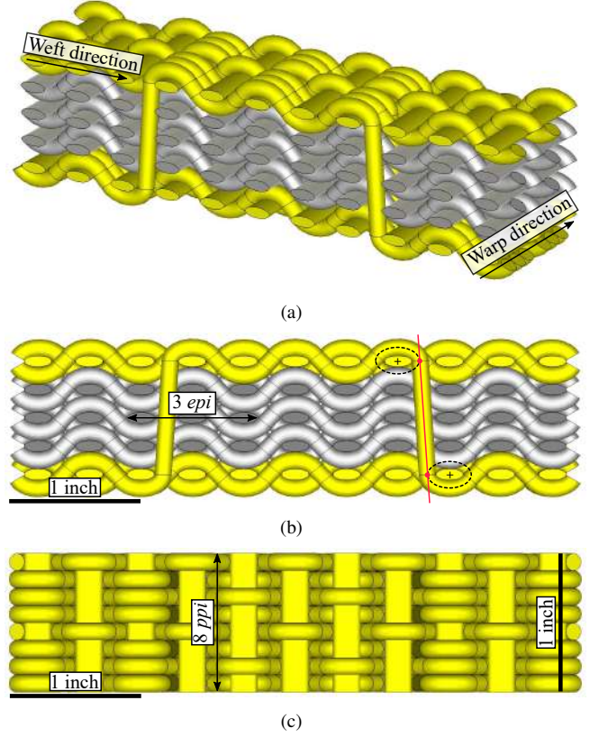
Figure 17: Generic multilayered woven structure using rigid warp threads and two materials, conductive (yellow) and dielectric (grey). (a) Woven structure overview. (b) Front view and epi parameter. (c) Top view and ppi parameter.
