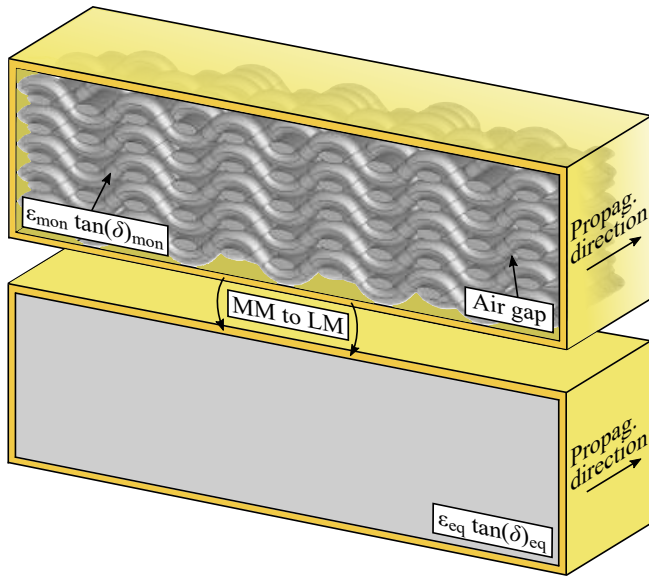
Figure 18: Translation from the MM into the LM outline applied to dielectric monofilaments using the waveguide based methodology.
