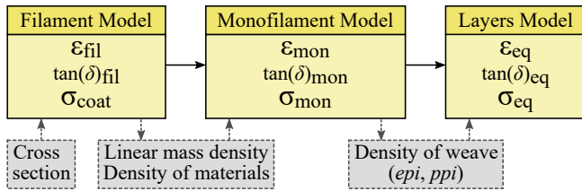
Figure 1: Three-step characterisation model, corresponding relative permittivities, loss tangents and electrical conductivities and required parameters for translation between models.
