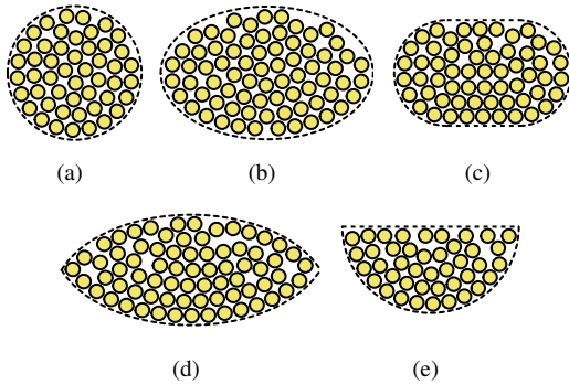
Figure 2: Different distributions of the filaments in the cross section of a multifilament thread. (a) Circular. (b) Pierce's elliptic. (c) Kemp's racetrack. (d) Hearle. (e) Bowshaped.
