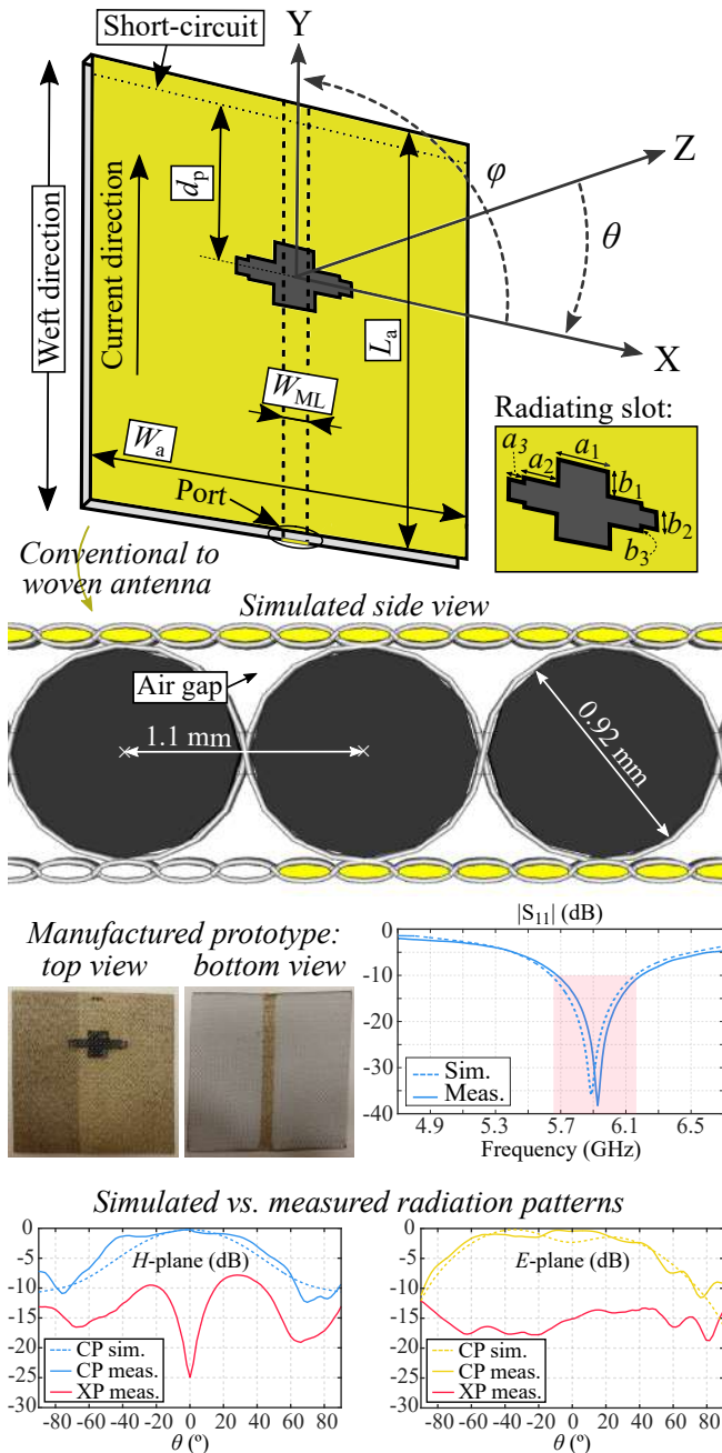
Figure 25: Overview of the development of the microstrip-fed slot antenna example [36].
