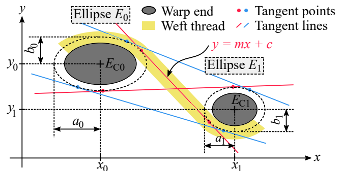
Figure 16: Generic mathematical modelling based on ellipses and tangents.
