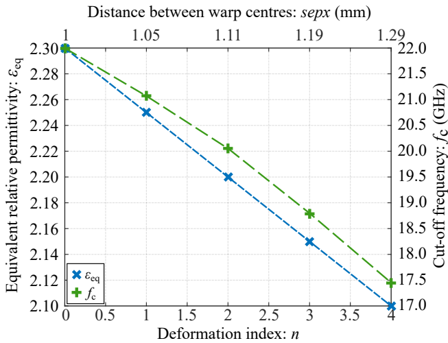
Figure 23: Modification of the \epsilon_{eq} and the f_c of a woven SIW depending on n and sepx .
