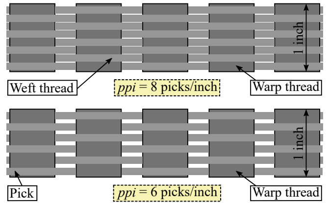
Figure 14: Schematic representation of the p_{pi} parameter (side view of the woven structure).
