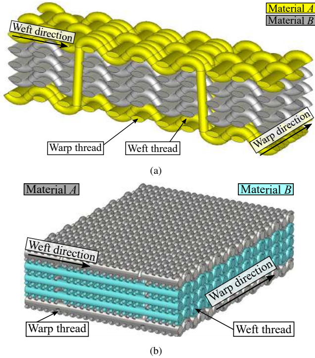
Figure 12: Generic multilayered woven structures using the MM and different materials. (a) Rigid warp threads. (b) Rigid weft threads.
