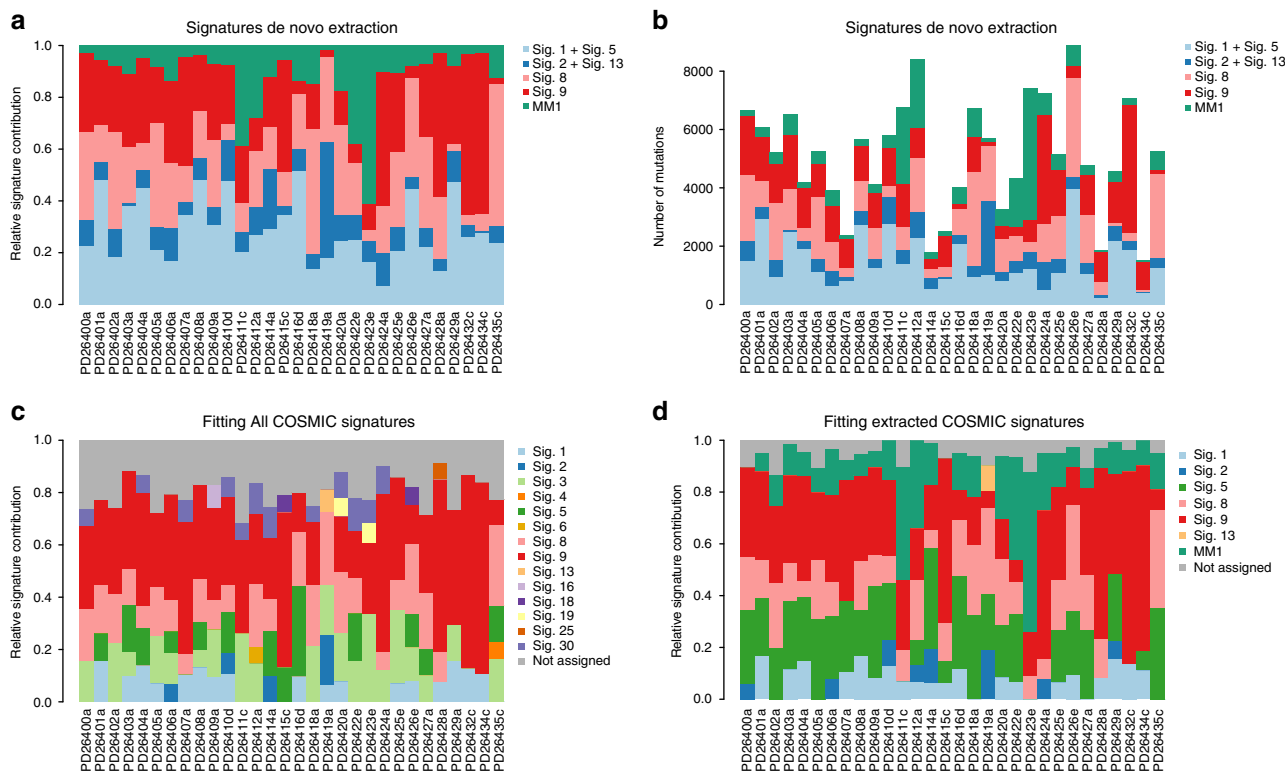
Fig. 1 Mutational signature de novo extraction vs. fitting. a, b The Alexandrov et al. NNMF framework 6,7 . From the 96-mutational classes, NNMF extracted the signatures' relative ( a ) and absolute ( b ) contribution among 30 MMs. c Running deconstructSig including all 30 COSMIC signatures several mutational processes were forced to be extracted (i.e., Signature 4). Furthermore, the new mutational process MM1 was not detected, being not included in the 30 COSMIC signatures. d Conversely, running the same fitting approach based on the mutational signature catalog extracted by NNMF, each signature contribution was better estimated for each patient. Sig. = signature
