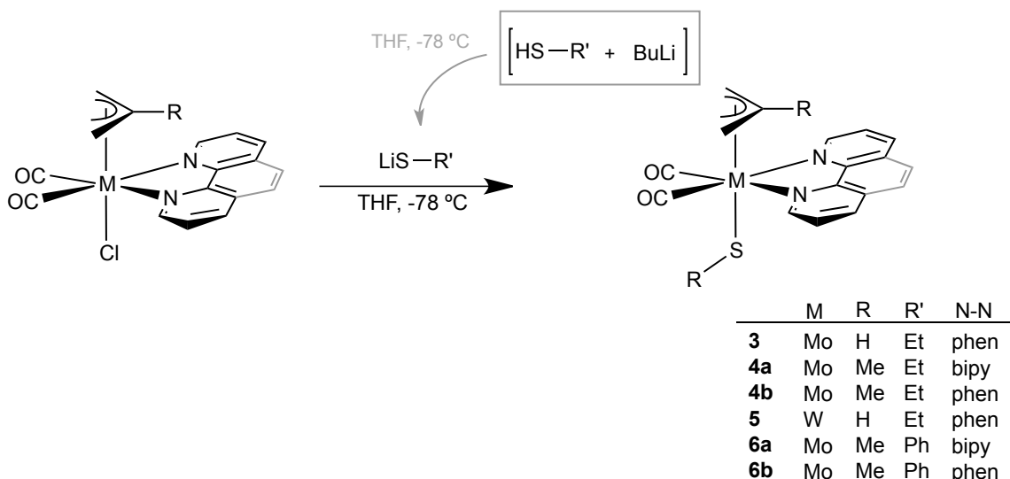
Scheme 2. Synthesis of thiolato complexes of [M(\eta^3\text{-allyl})(\text{CO})_2(\text{N-N})] fragments.
