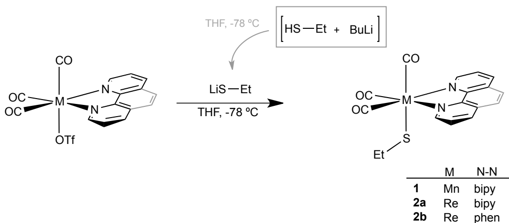
Scheme 1. Synthesis of ethylthiolato complexes [M(SET)(CO)_3(N-N)] .
