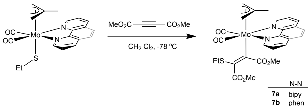
Scheme 3. Reactivity of [\text{Mo}(\eta^3\text{-methylallyl})(\text{SEt})(\text{CO})_2(\text{N-N})] ( 6a,b ) compounds towards DMAD.
