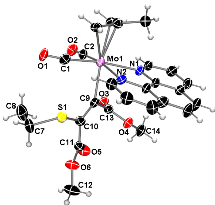
Figure 3. Molecular structure of the insertion product 7b , displaying thermal ellipsoids at 30 % probability level.
