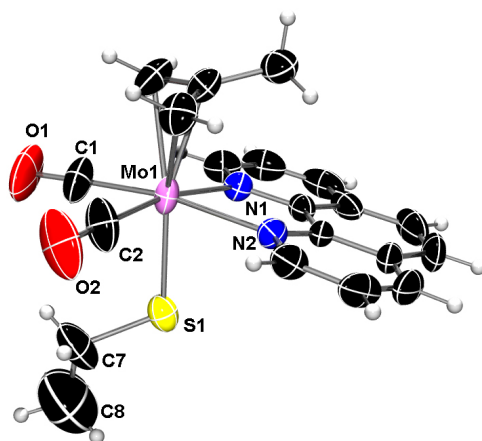
Figure 2. Molecular structure of compound 4b , displaying thermal ellipsoids at 30 % probability level.
