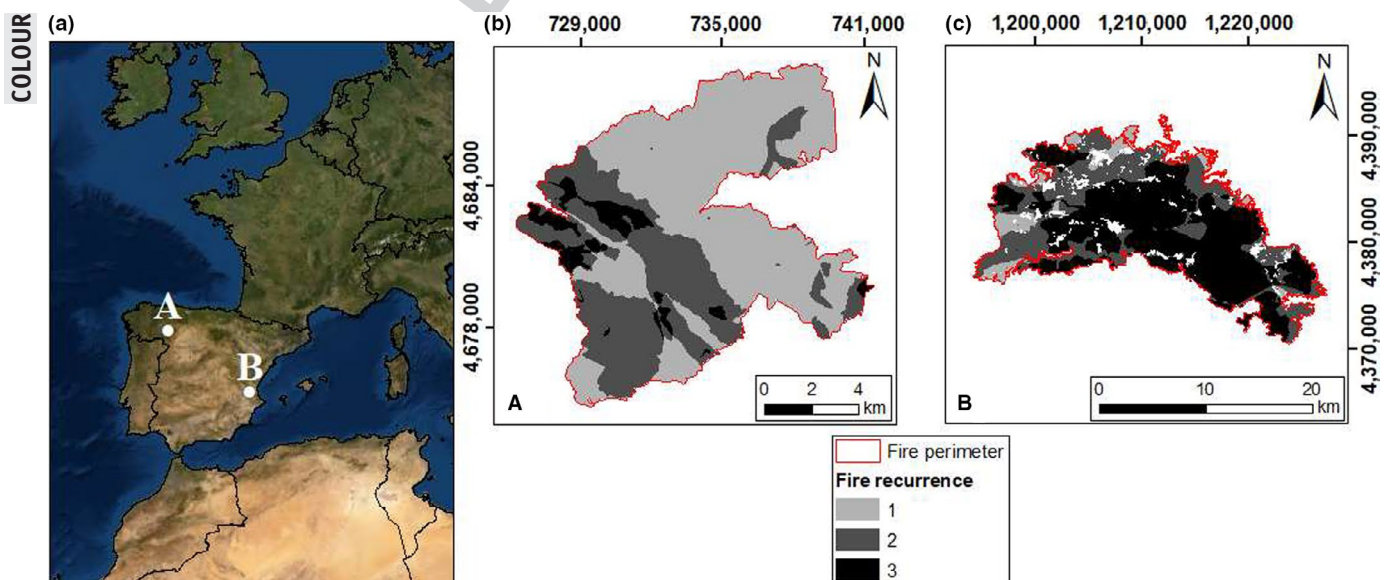
FIGURE 1 Location (ESRI, 2019) (a) and fire recurrence (b and c) for the period 1978–2012 of Sierra del Teleno (A) and Cortes de Pallás (B) wildfires. Fire recurrence maps were computed through visual interpretation of Landsat imagery covering the study period
