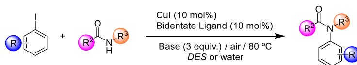
Scheme 1. CuI-catalyzed Goldberg-type C–N coupling of aryl iodides with primary/secondary amides under air in DES or aqueous media.
