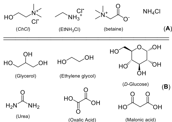
Figure 1. Hydrogen-bond-acceptors (HBA, top) and hydrogen-bond-donors (HBD, down) usually employed in the synthesis of sustainable Deep Eutectic Solvents (DESs).
