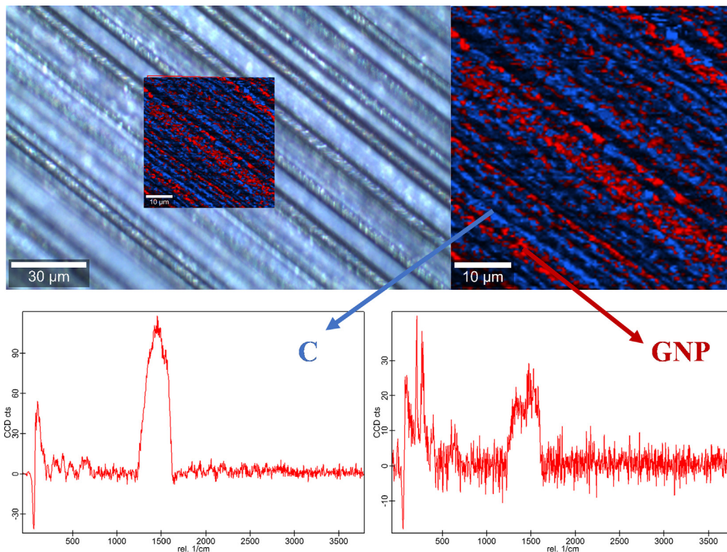
Fig. 7. Raman spectra mapping of the wear surface lubricated with the nanolubricant of GNP.
