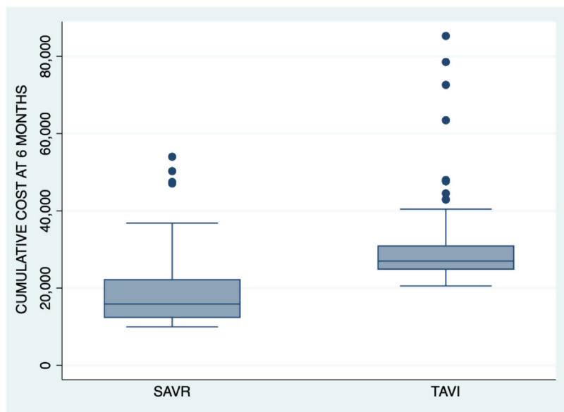
Fig. 2. Boxplot. Cumulative cost at 6 months.
