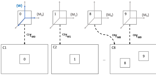
Fig. 4. Schematic mapping system transformations. Where \{M_0\} , \{M_1\} , \{M_8\} , \{M_9\} are the coordinate systems of the markers in 3D space and C1, C2 y C8 are the cameras that take the images of the markers. In this case, world reference frame is set on marker with id 0.
