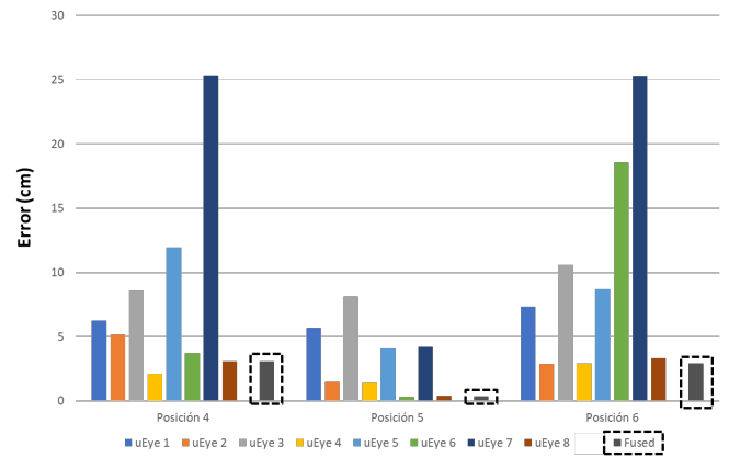
Fig. 9. Comparison between the final position of the robot and the intermediate estimates of the 8 cameras. Data from 3 of the previously fixed positions for the robot that can be seen in Fig. 8.
