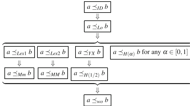
Fig. 3 Relations between orders
