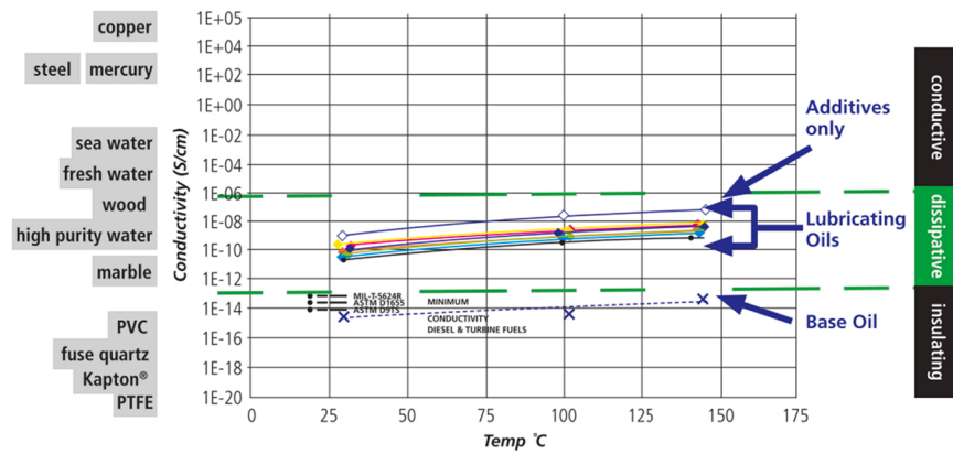
Fig. 1. Electrical conductivity in ATFs [5].
