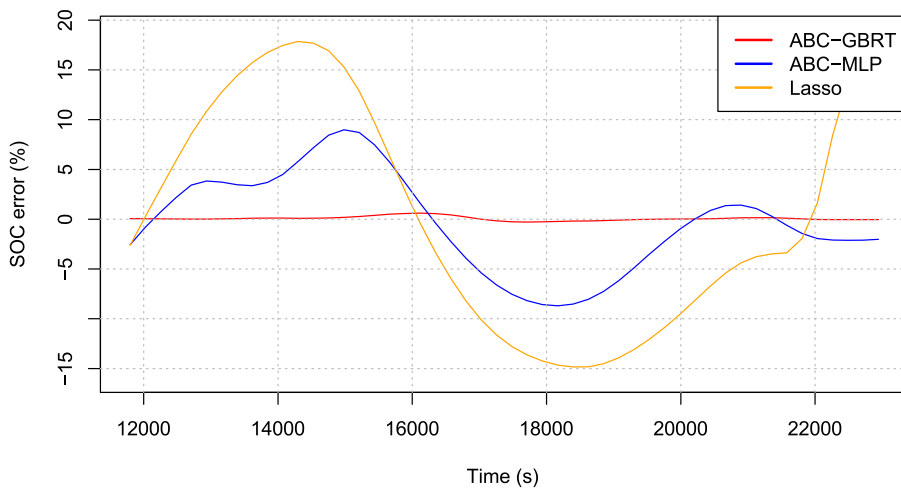
Fig. 10. Absolute error of ABC/GBRT, ABC/MLP and LASSO.
