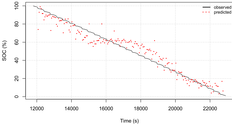
Fig. 3. Observed and predicted SOC results (100% to 0%) for the ABC/MLP model.
