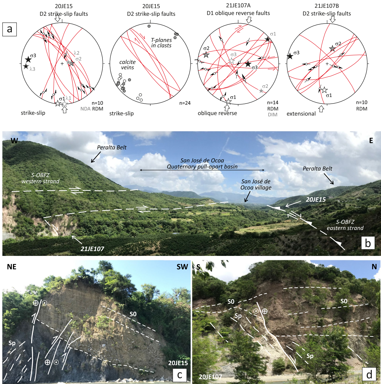
Figure 11. Structural analysis of S-OBFZ segment. (a) Stereoplots of the principal stress-axes obtained from inversion of fault-slip data (see Supporting Information S3 and S4). (b) View looking N of the Quaternary San José de Ocoa pull-apart basin, limited by the eastern and western strands of the S-OBFZ segment. (c) Tectonic contact between the folded and faulted mudstones of the Numero Fm and the gravels and sands of the basin through a subvertical fault system of oblique reverse right-lateral slip movement. Note the westward tilting of the Quaternary deposits. (d) Tectonic contact between the folded limestones of the Jura Fm with the poorly consolidated subhorizontal conglomerates of the basin.
