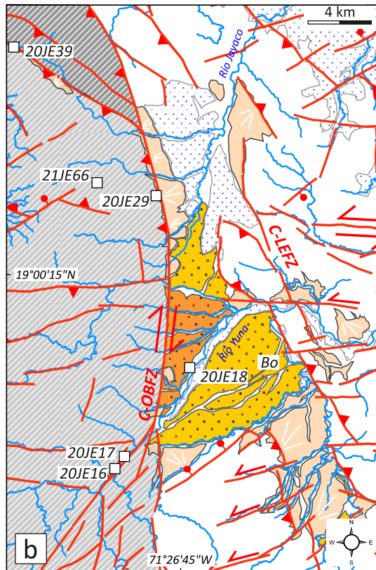
Figure 12. Structural analysis of C-OBZ segment. (a) Stereoplots of the principal stress-axes obtained from inversion of fault-slip data (see Supporting Information S3 and S4). (b) Structural map of the C-OBZ segment and the Quaternary Bonao basin. Bo, Bonao village. (c) View looking W of the Cordillera Central mountain front formed by the C-OBZ near the Bonao village. Note the sharp edge to the topography, the perched valleys and the triangular facets. (d) Panoramic view of the thrust contact between the volcanic rocks of the Tireo Group in the hanging-wall block, the Quaternary alluvial fans and the metamorphic Duarte Complex in the footwall block.
