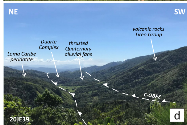
Figure 12. Structural analysis of C-OBZ segment. (a) Stereoplots of the principal stress-axes obtained from inversion of fault-slip data (see Supporting Information S3 and S4). (b) Structural map of the C-OBZ segment and the Quaternary Bonao basin. Bo, Bonao village. (c) View looking W of the Cordillera Central mountain front formed by the C-OBZ near the Bonao village. Note the sharp edge to the topography, the perched valleys and the triangular facets. (d) Panoramic view of the thrust contact between the volcanic rocks of the Tireo Group in the hanging-wall block, the Quaternary alluvial fans and the metamorphic Duarte Complex in the footwall block.
