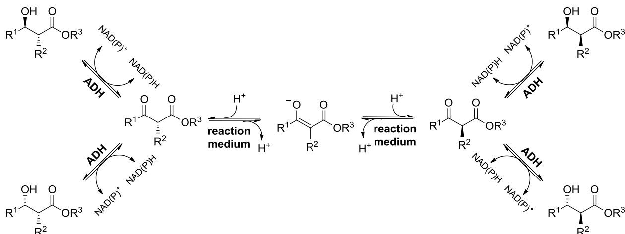
Scheme 1. ADH-catalysed reduction of \alpha -substituted \beta -ketoesters to afford a mixture of two diastereomeric pairs of alcohols through base-catalysed racemisation.
