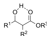
Figure 2. Intramolecular H-bond interaction in \beta -hydroxyesters 2 or 3 .
